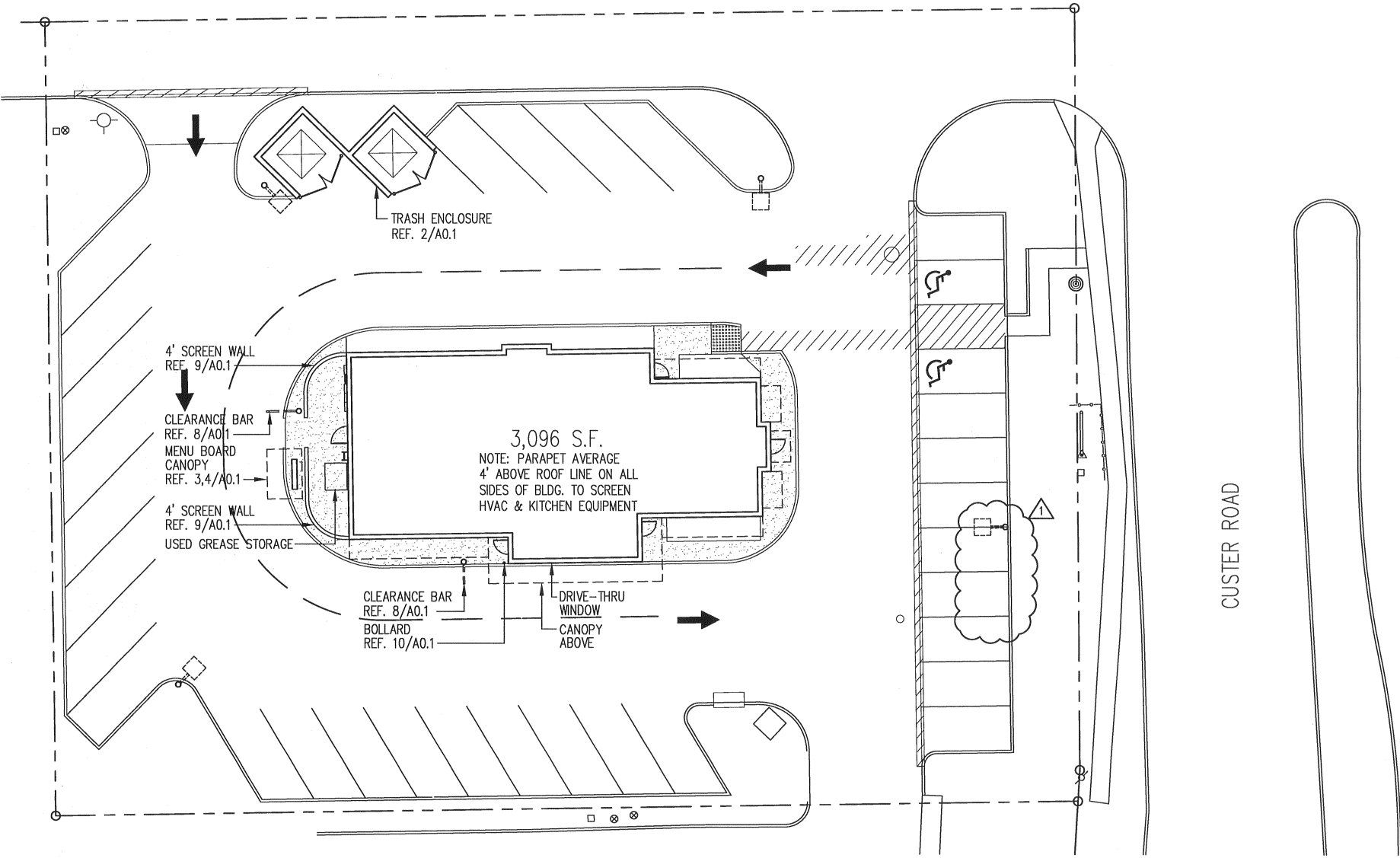
1 SITE PLAN SCALE: 1"=20' N
